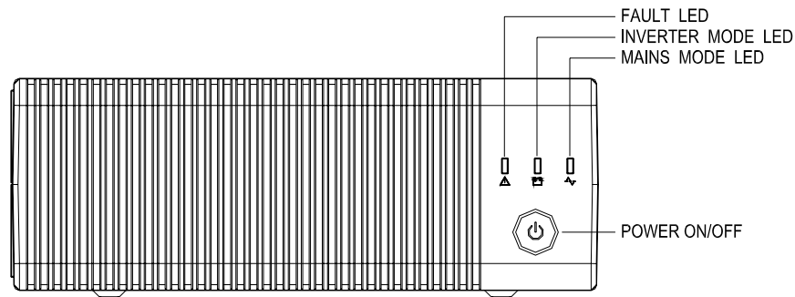
Figure 1 Front Panel
