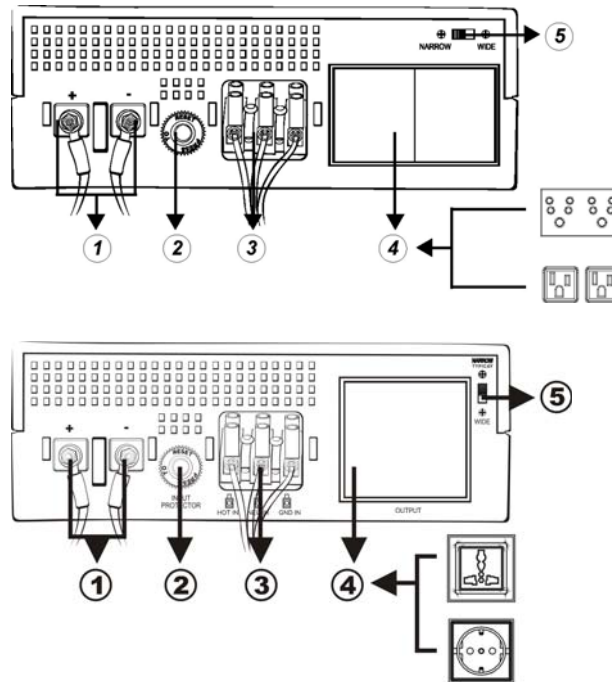
Figure 2 Back Panel
