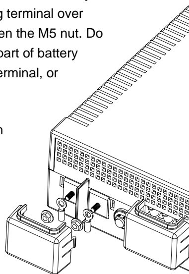
Figure 4 Battery Cable Connection to Inverex
